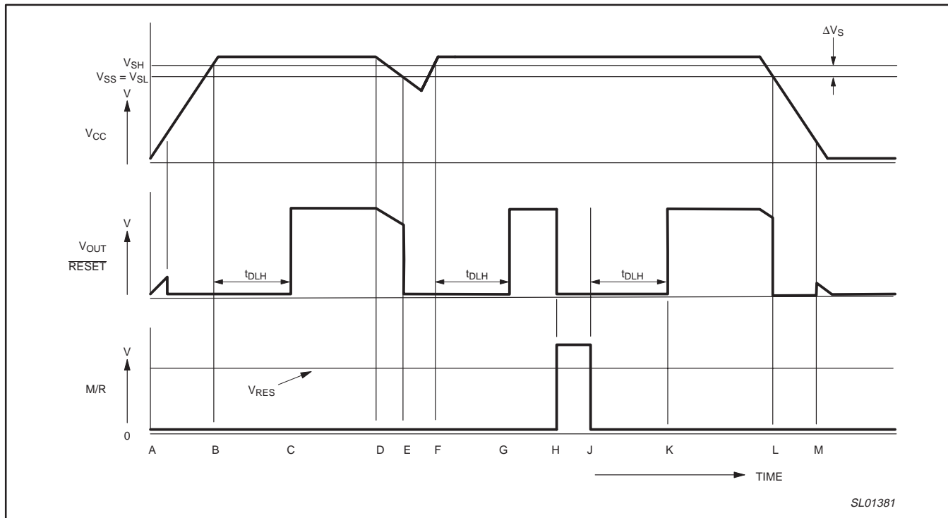
Figure 17. Timing diagram.
