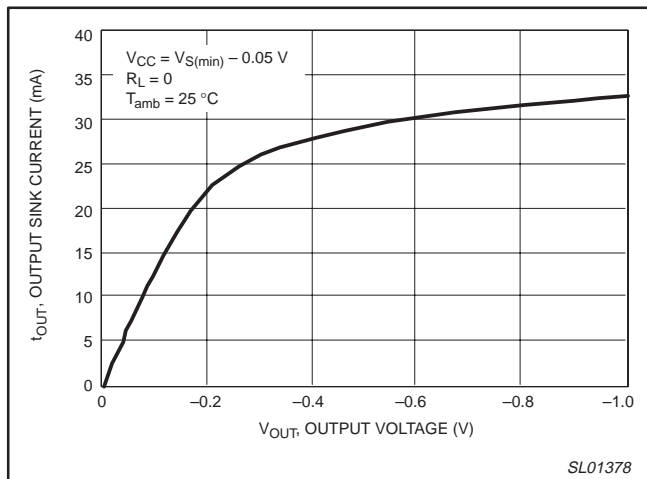
Figure 15. Output sink current versus output voltage.
