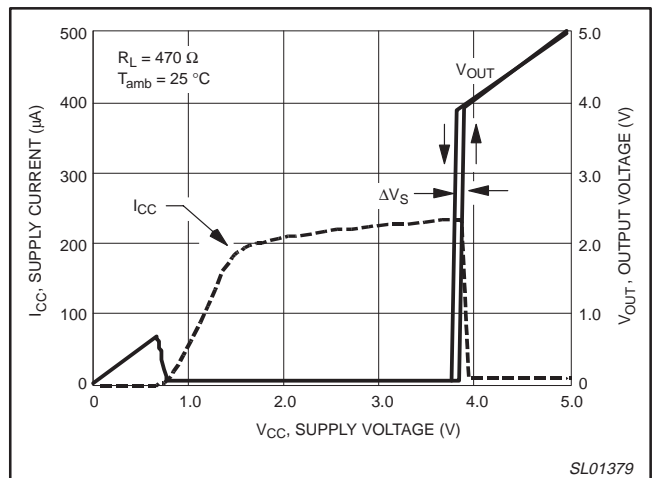
Figure 14. ICC and VOUT versus supply voltage.
